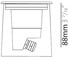
Slim Housing L9A09500
