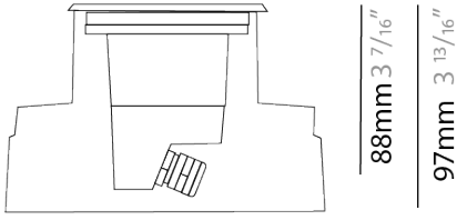
Wide Housing L9A09500
